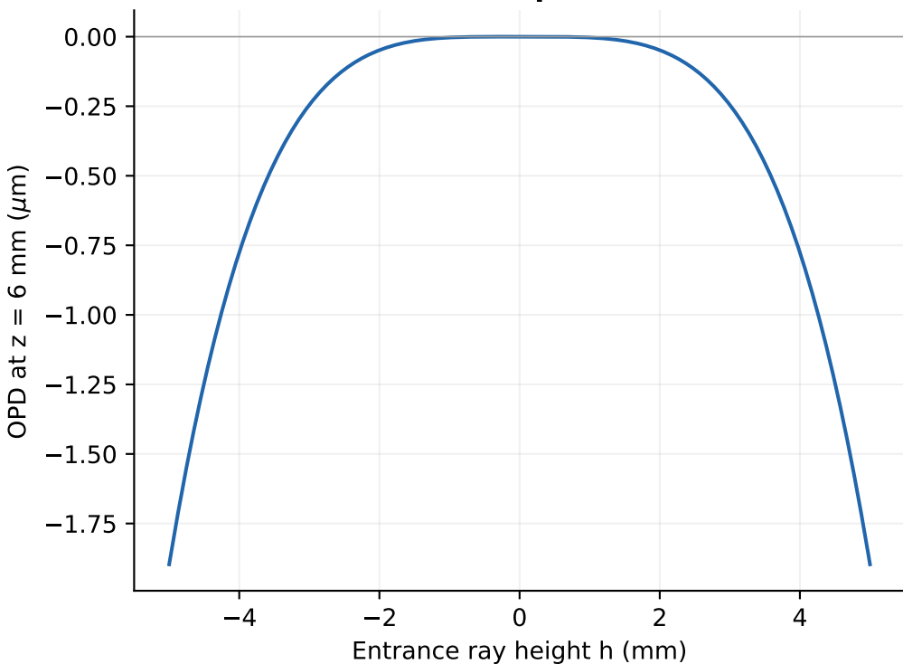
OPD relative to paraxial focus
